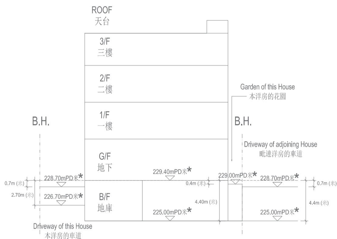
Section B 剖面圖B
